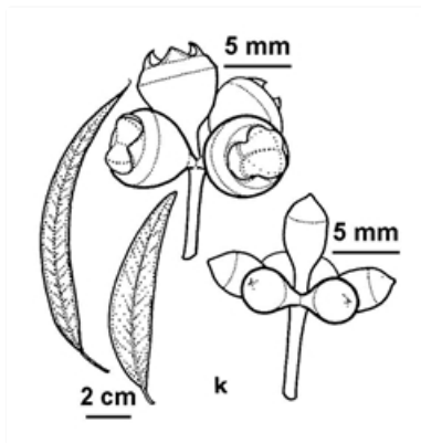
Line drawings. k. juvenile (right) and adult (left) leaves; buds and gumnuts. KR Thiele, Australian National Herbarium © 2021 Royal Botanic Gardens Board, Melbourne, Vic
